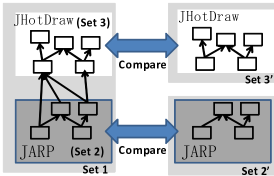
Figure 3. Analysis Overview
