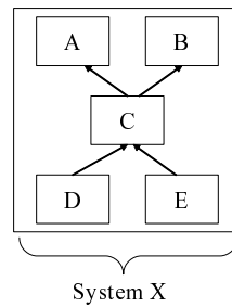
Figure 1. Component Graph
