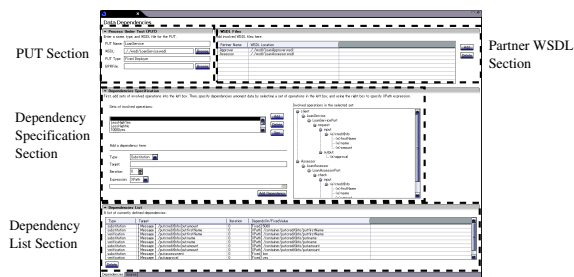
Figure 7: BPEL Data Dependency Editor
