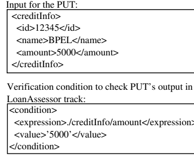
Figure 3: Example of Test Data
