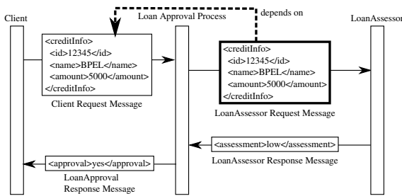
Figure 4: Example of Data Dependency
