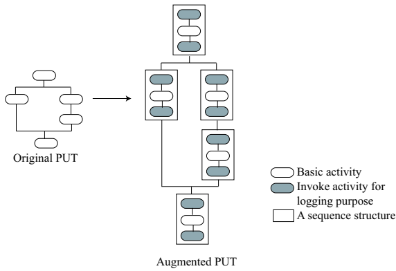
Figure 5: Augmentation of the PUT
