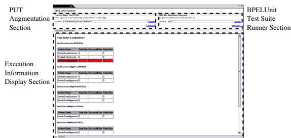
Figure 8: BPELUnit Runner Editor
